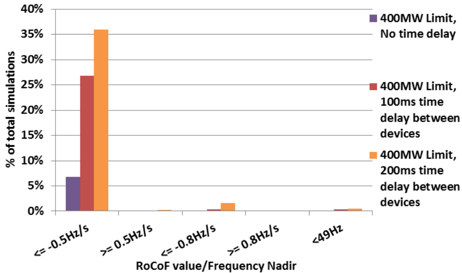
Figure 7.1-2: Variation in the time of the synthetic inertia injection, limited to 400 MW - Percentage of cases where RoCoF exceeds a value and frequency nadir is below 49 Hz.
