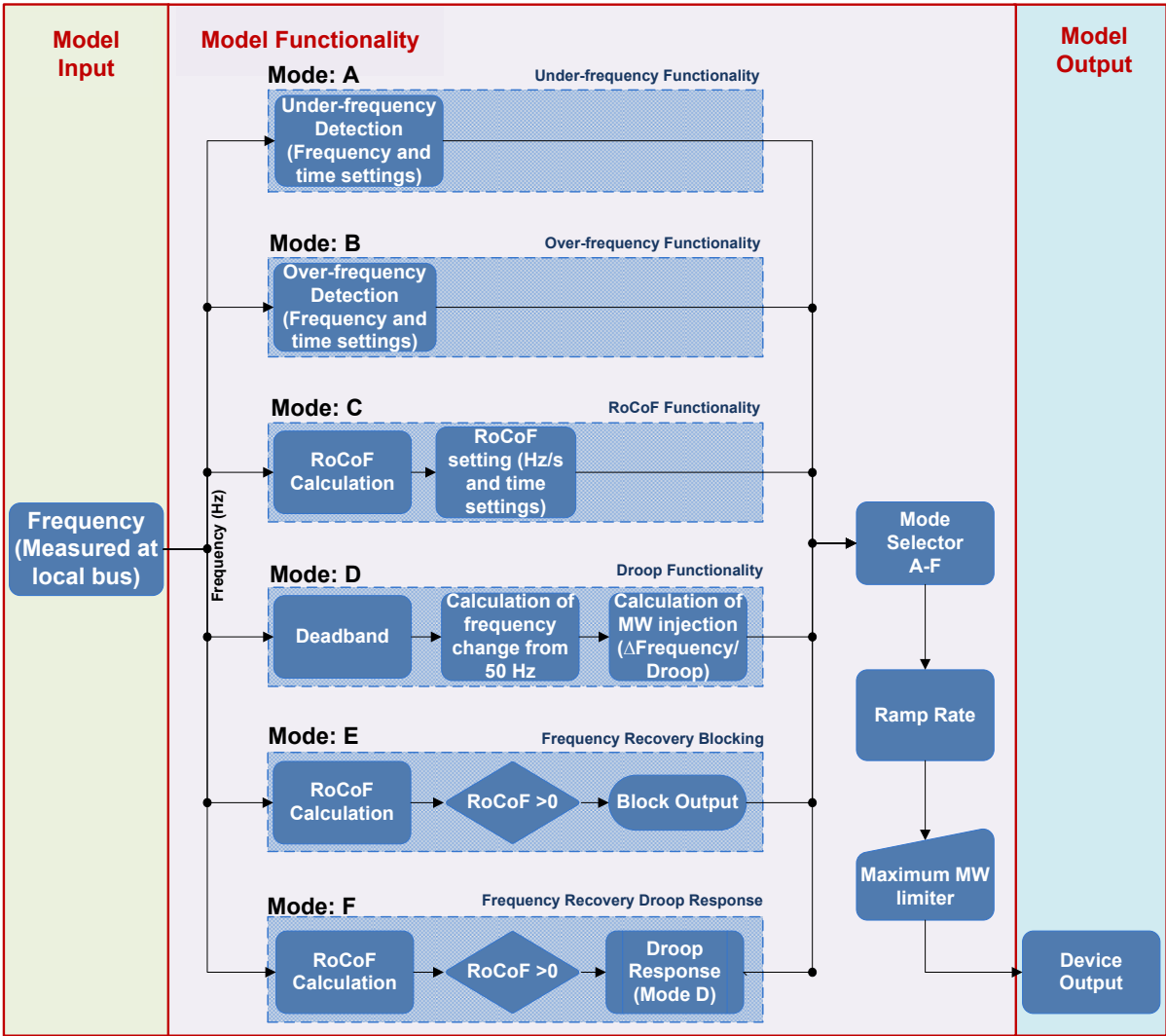
Figure 3.3-2: Simplified functionality overview of the synthetic inertia device model.
