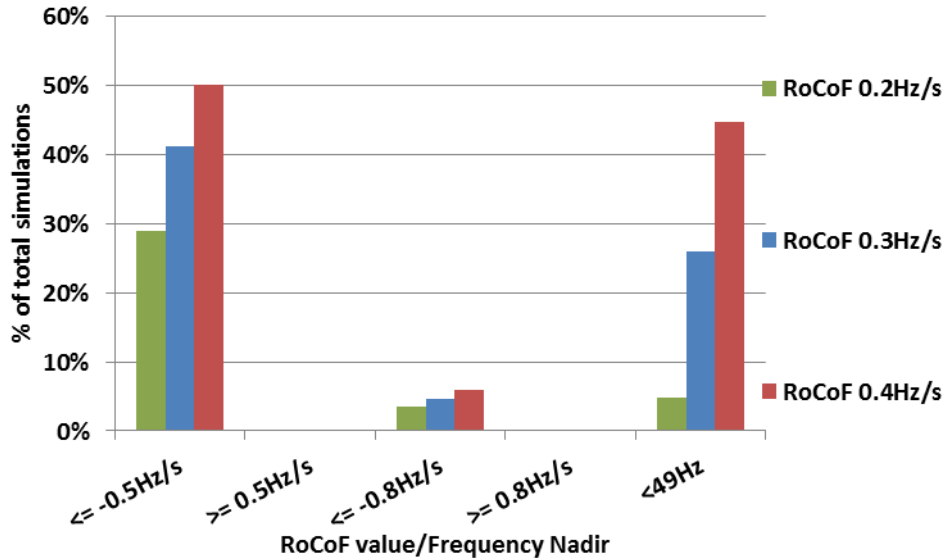
Figure 4.4-6: Synthetic inertia response while the defined RoCoF threshold is exceeded, no active power limit - Percentage of cases where RoCoF exceeds a value and frequency nadir is below 49Hz.
