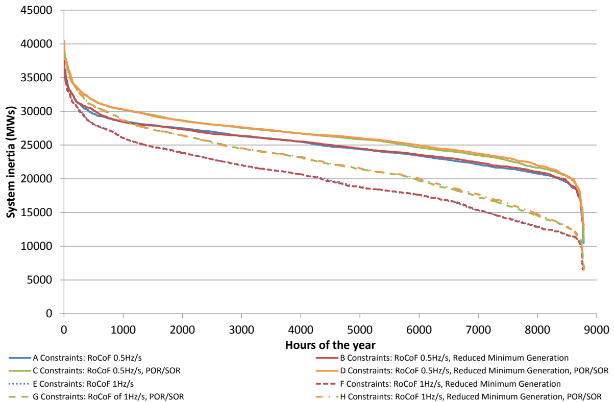
Figure 4.1-1: Duration curves for each of the eight techno-economic studies.
