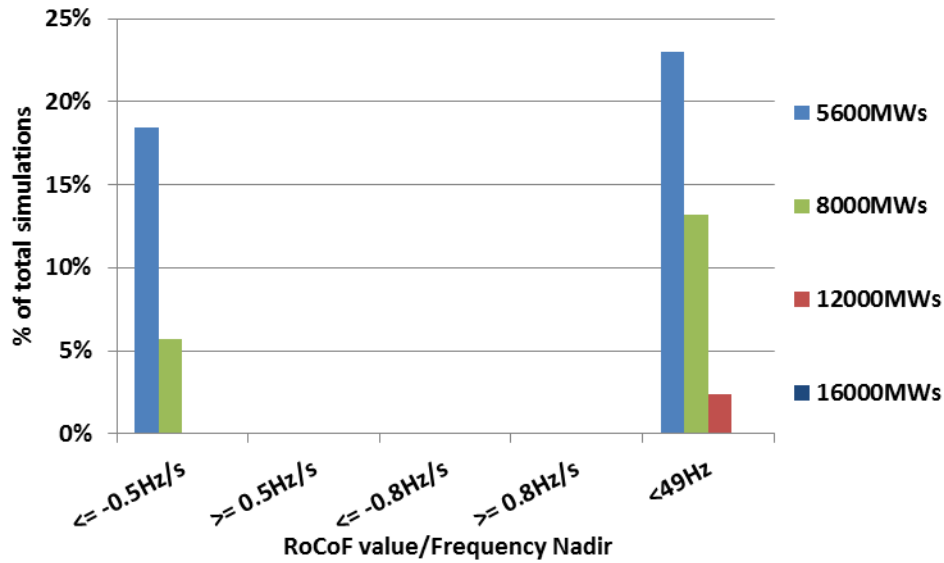
Figure 4.3-1: Synchronous inertia - Percentage of cases where RoCoF exceeds a value and frequency nadir is below 49Hz.
