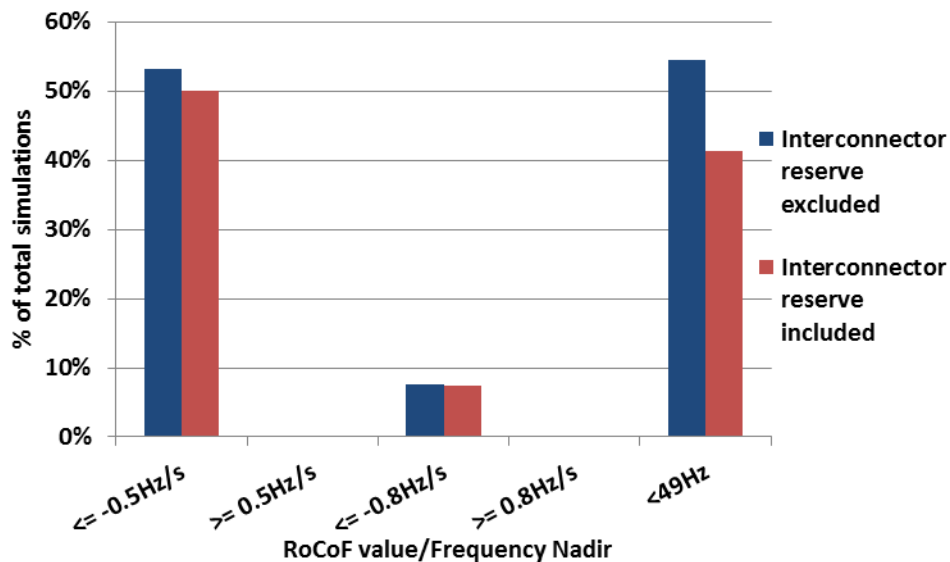
Figure 4.2-1: Basecase - Percentage of cases where RoCoF exceeds each setpoint and frequency nadir is below 49 Hz.
