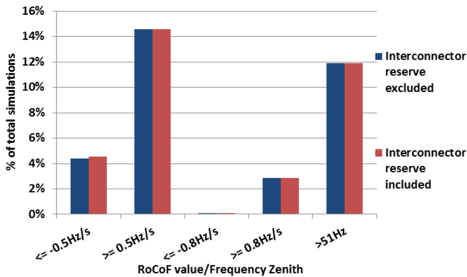
Figure 4.2-2: Over-frequency basecase - Percentage of cases where RoCoF exceeds each setpoint and frequency zenith is above 51 Hz.
