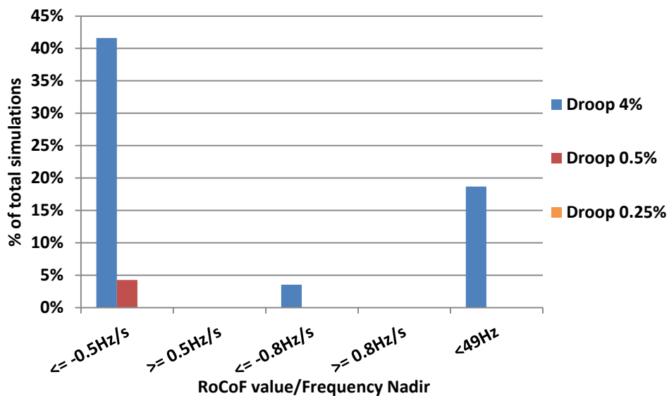
Figure 4.4-10: Droop-control sensitivity - Percentage of cases where RoCoF exceeds a value and frequency nadir is below 49Hz
