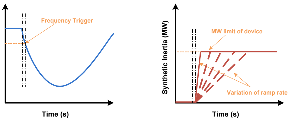
Figure 3.3-7: Control Mode A, Stepped response at different ramp rates of the supplementary inertia.
