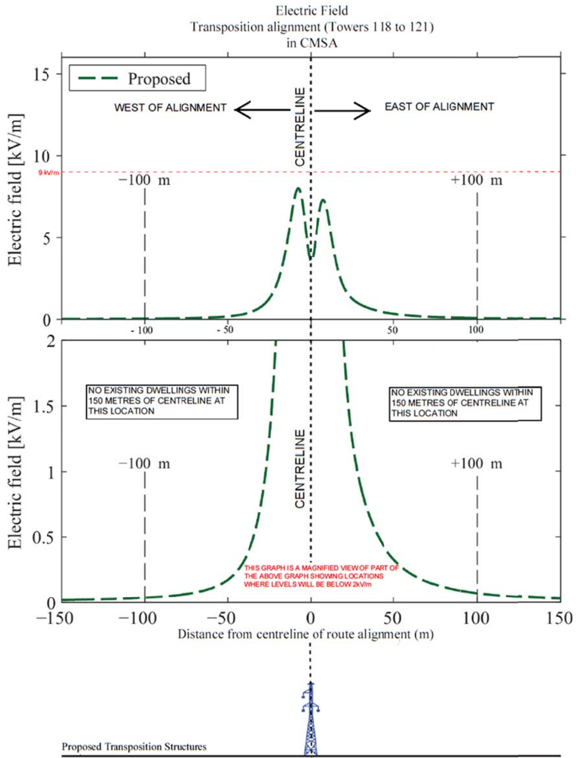
Figure 5.6: Calculated Electric Field Profile for the Proposed Transposition Tower Configuration
