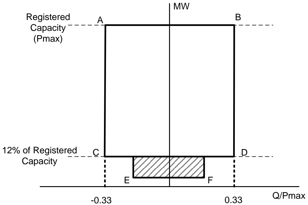
Figure WFPS PPM 1.4 – Minimum Reactive Power Capability of Controllable Controllable PPM
