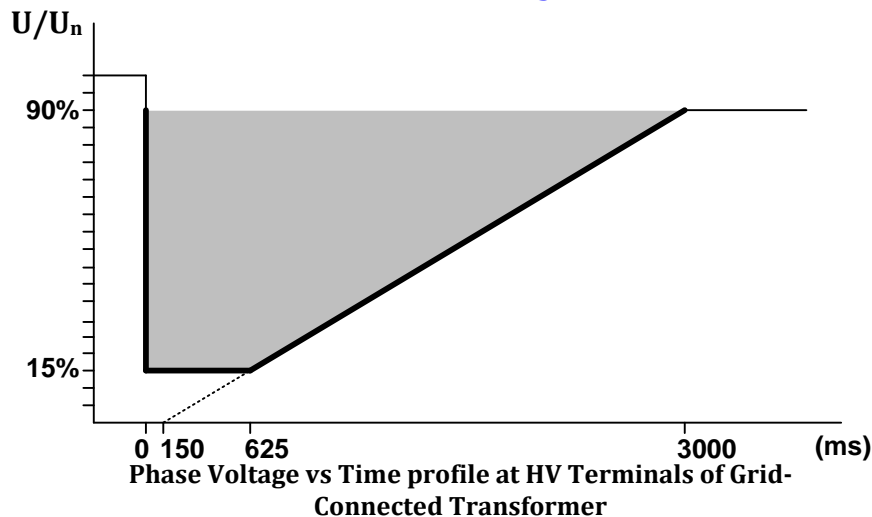
Figure WFPS1.1 - Fault Ride-Through Capability of Controllable WFPSs Controllable PPMs
